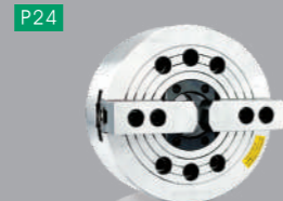
NT-200 (不含連接板) 二爪中空油壓夾頭 2-jaw through-hole power chuck, (adapter excluded)
